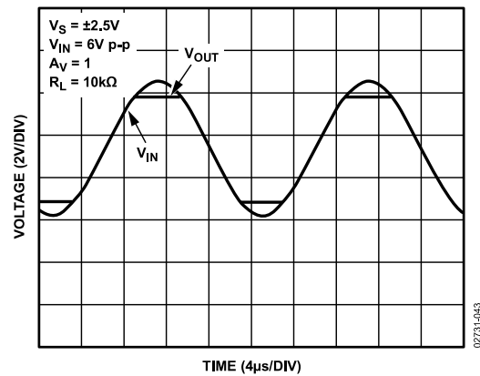
Figure 44. No Phase Reversal
