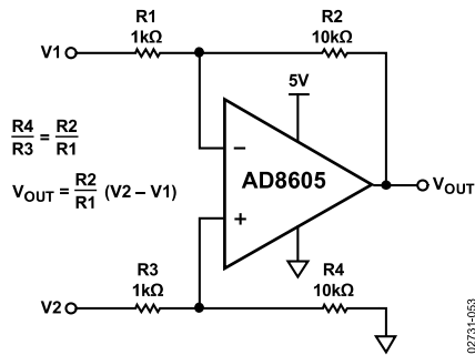
Figure 54. Difference Amplifier, A_v = 10
