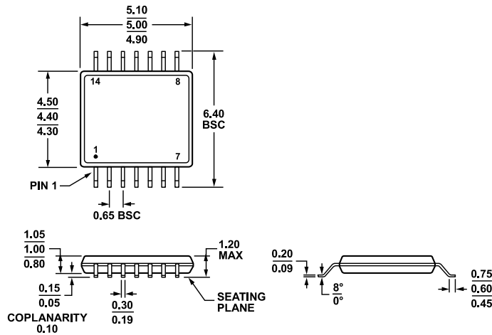
COMPLIANT TO JEDEC STANDARDS MO-153-AB-1 Figure 64. 14-Lead Thin Shrink Small Outline Package [TSSOP] (RU-14) Dimensions shown in millimeters and (inches)
