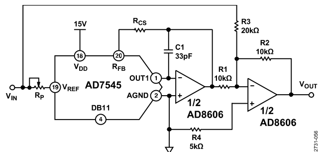
Figure 57. Bipolar Operation
