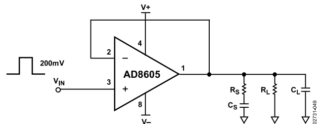
Figure 49. Snubber Network Configuration
