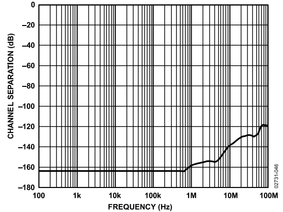
Figure 47. Channel Separation vs. Frequency
