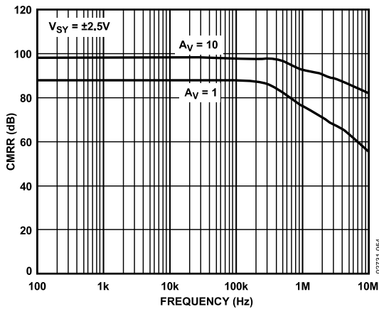
Figure 55. Difference Amplifier CMRR vs. Frequency
