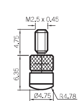
Ø4.75mm Dome
