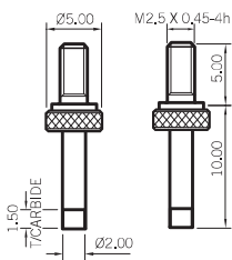
Ø2.00mm Pin
