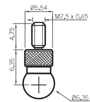
Ø6.35mm Ball
