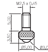
Ø3.00mm Ball
