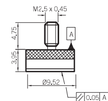
Ø9.52mm Flat
