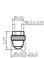
Ø3.00mm Ball
