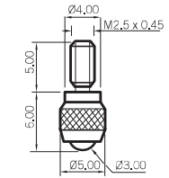
Ø3.00mm Ball
