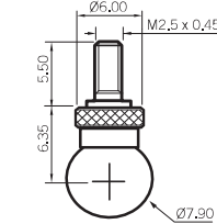
Ø7.90mm Ball
