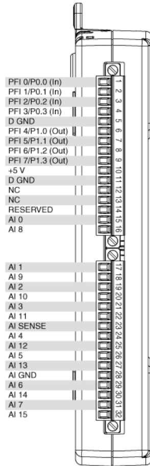
USB-6210 Pinout
