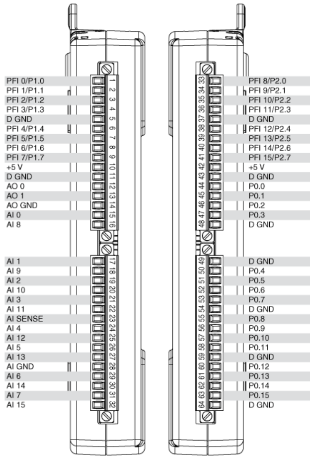
USB-6212/6216 Pinout
